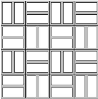
laying scheme 6
