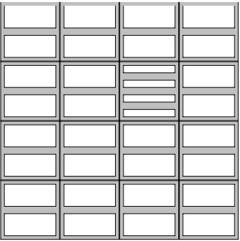
laying scheme 4
