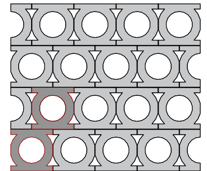
laying scheme 1 17,36 pcs / sqm
